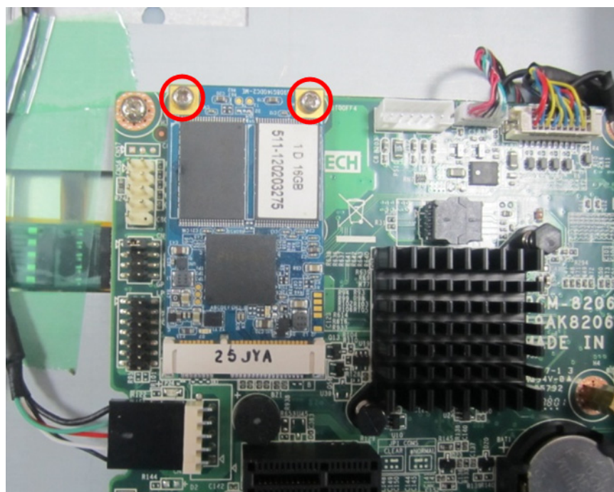
Figure 2.14 Installing mSATA
