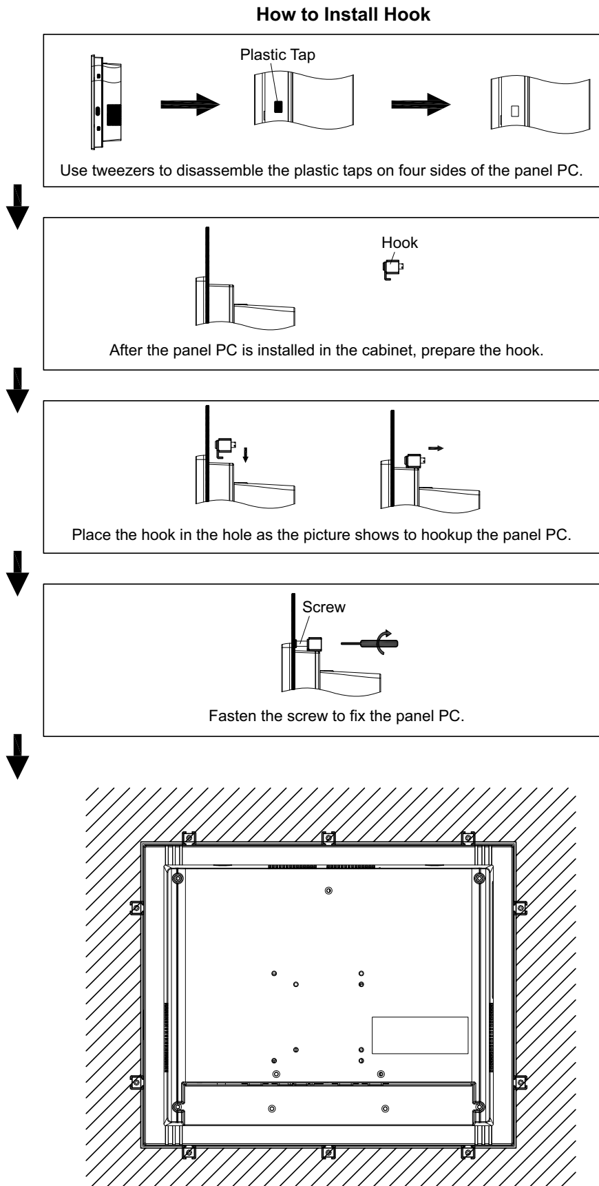
Figure 2.27 Installing Hook
