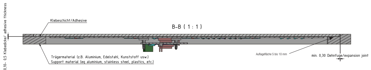
Cross section when inserting (without protection plate)
