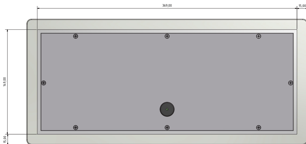
View from below (with protection plate)
