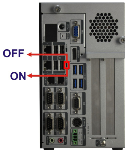
Figure 3-7: ACC Mode Switch
