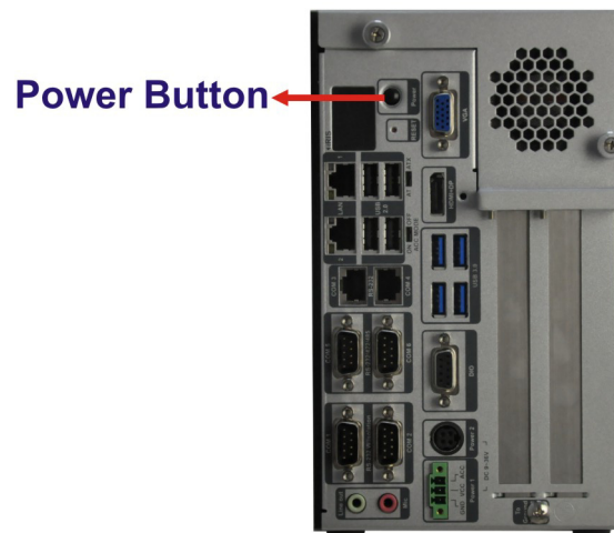
Figure 3-27: Power Button
