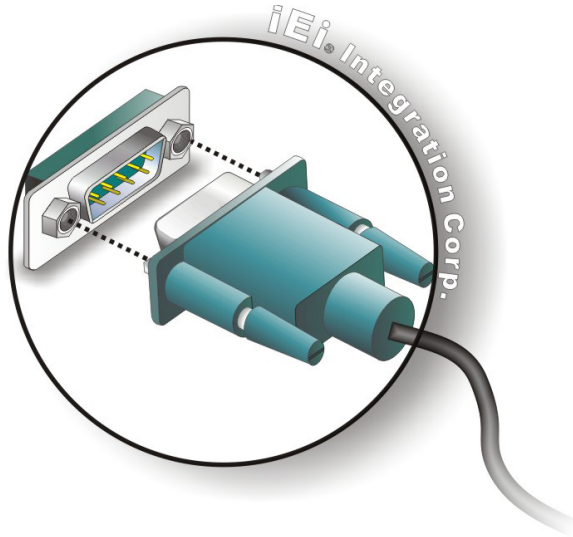
Figure 3-18: Serial Device Connector
