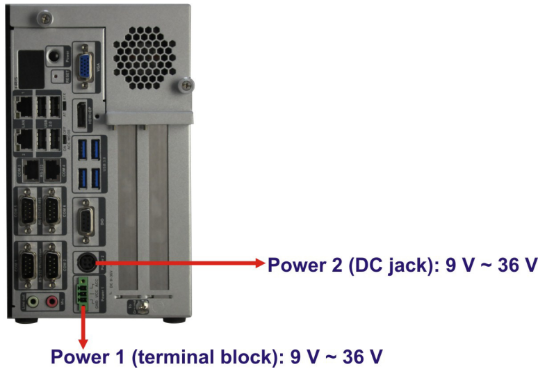
Figure 3-28: Power Connectors
