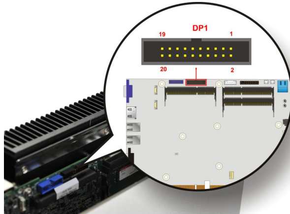
Figure 3-23: Internal DisplayPort Connector Location
