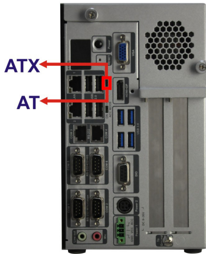
Figure 3-8: AT/ATX Power Mode Switch
