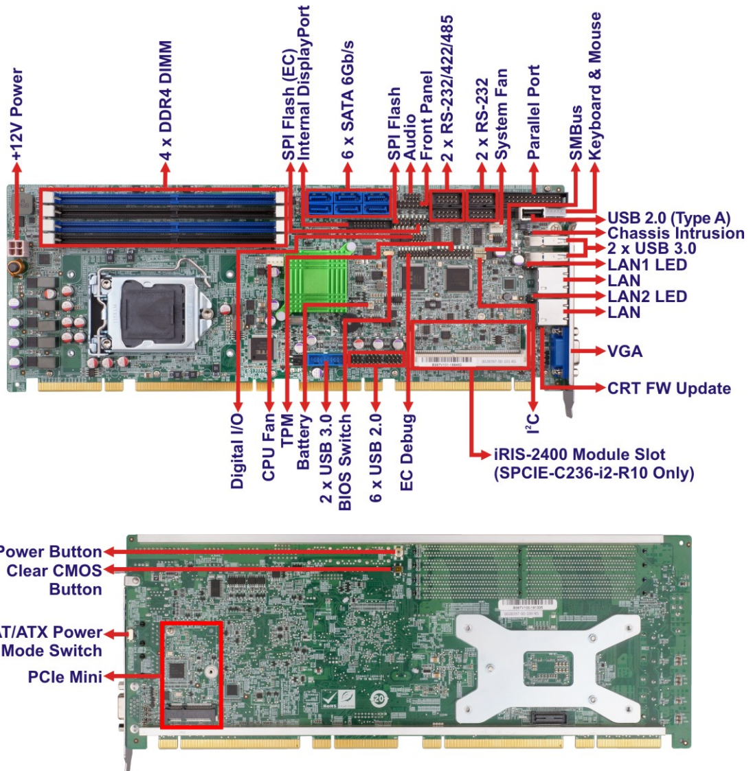
Figure 1-2: Connectors
