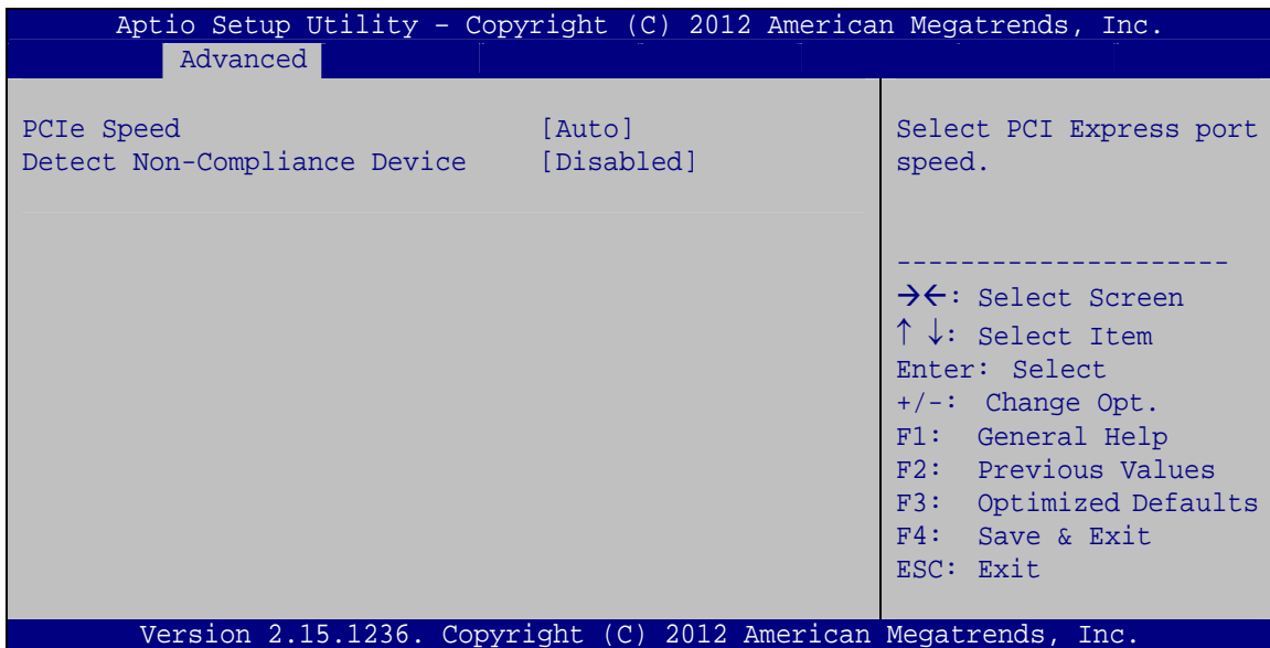
BIOS Menu 20: PCIEX4_1 Slot Configuration Menu
