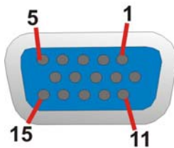
Figure 3-32: VGA Connector
