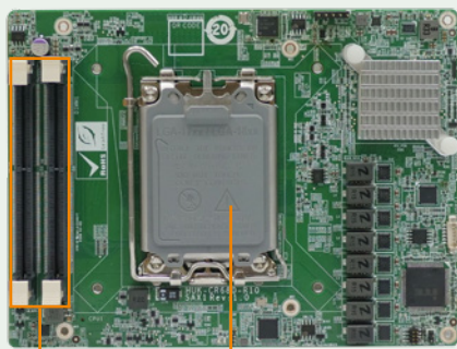
2 x DDR4 3200 SO-DIMM (up to 64 GB)
