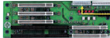
PICMG1.0 Form Factor Backplane
