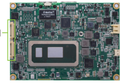
▲ Rear view
